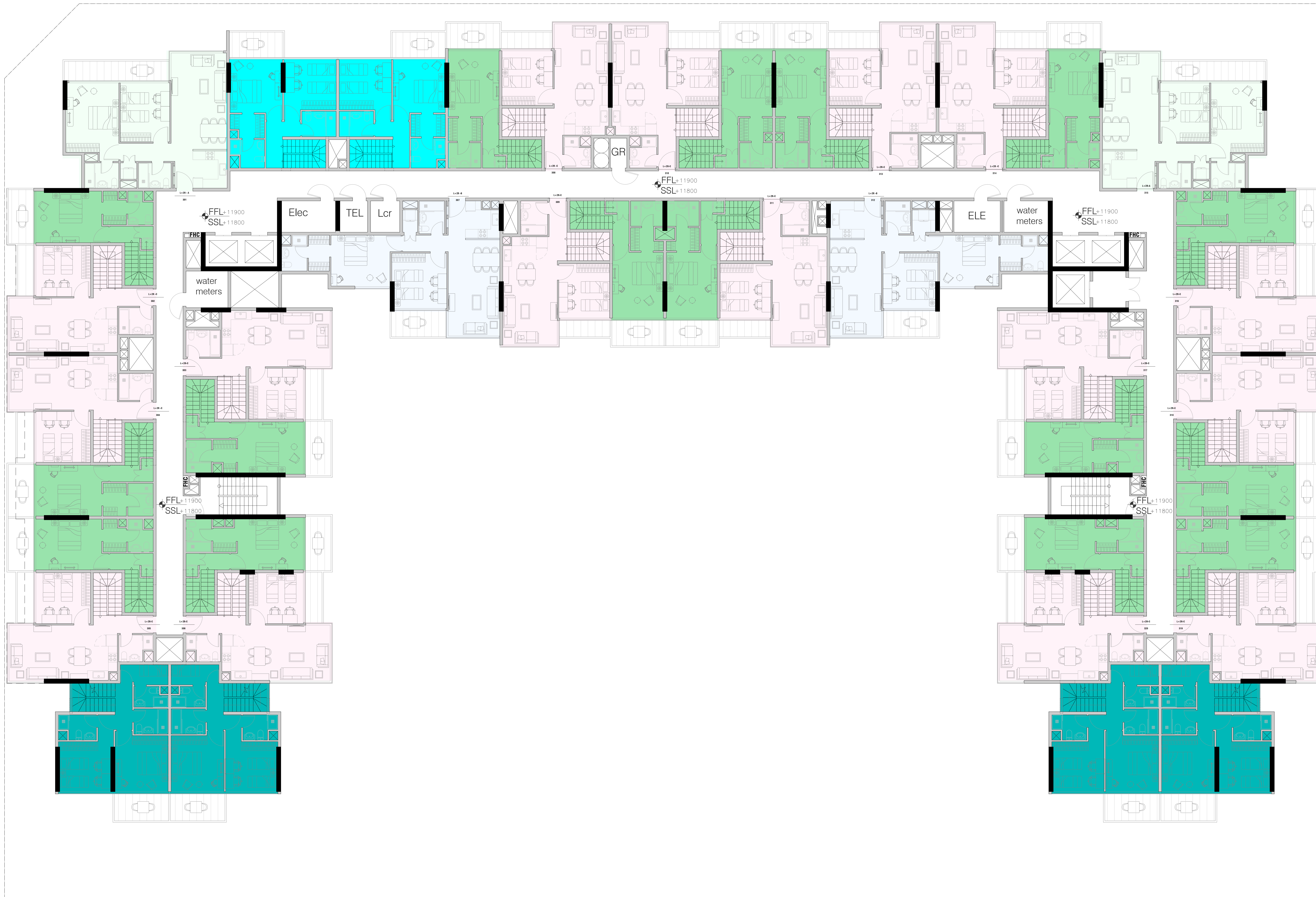
THIRD FLOOR PLAN
